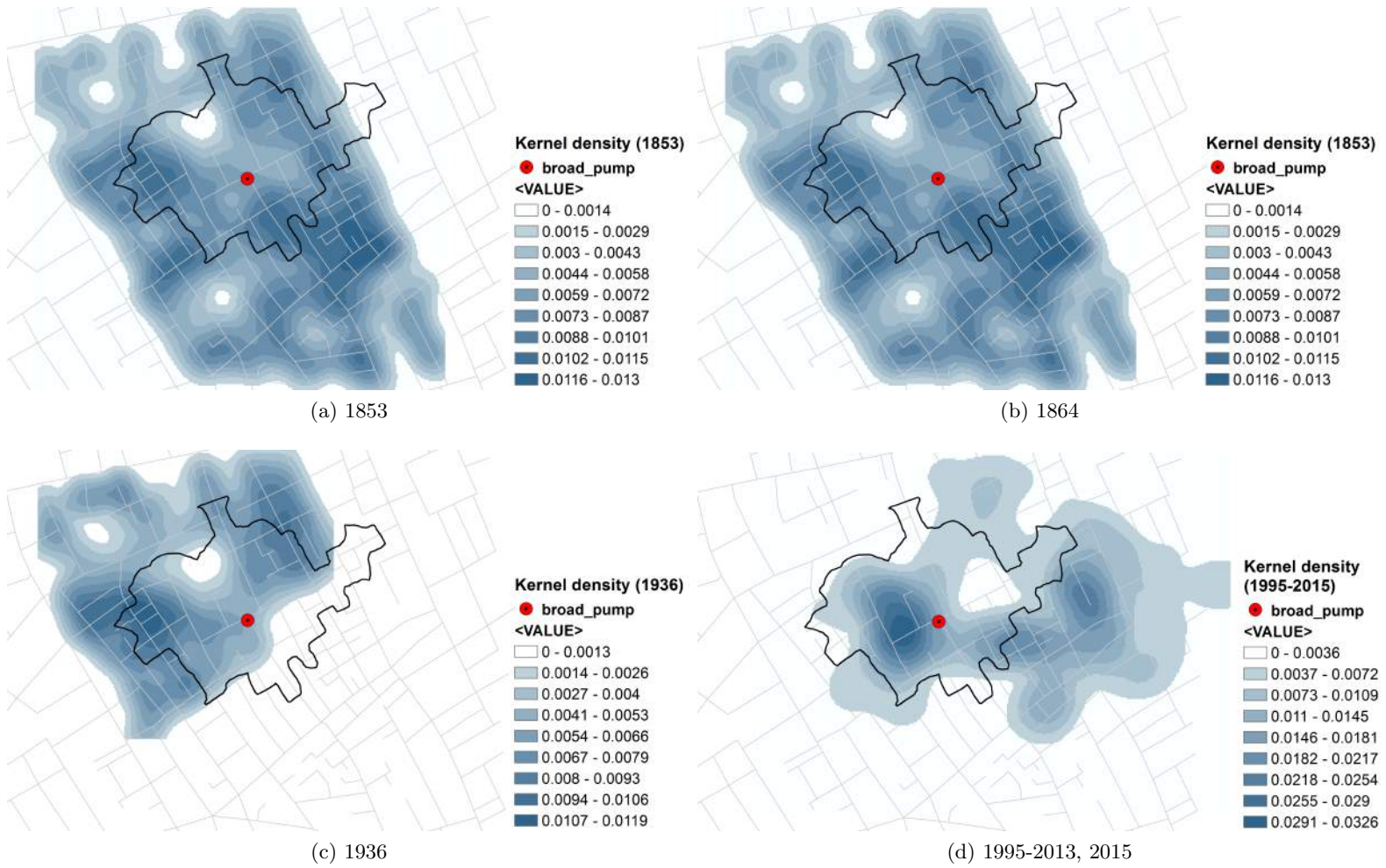
Figure B1: Kernel Density Estimates
