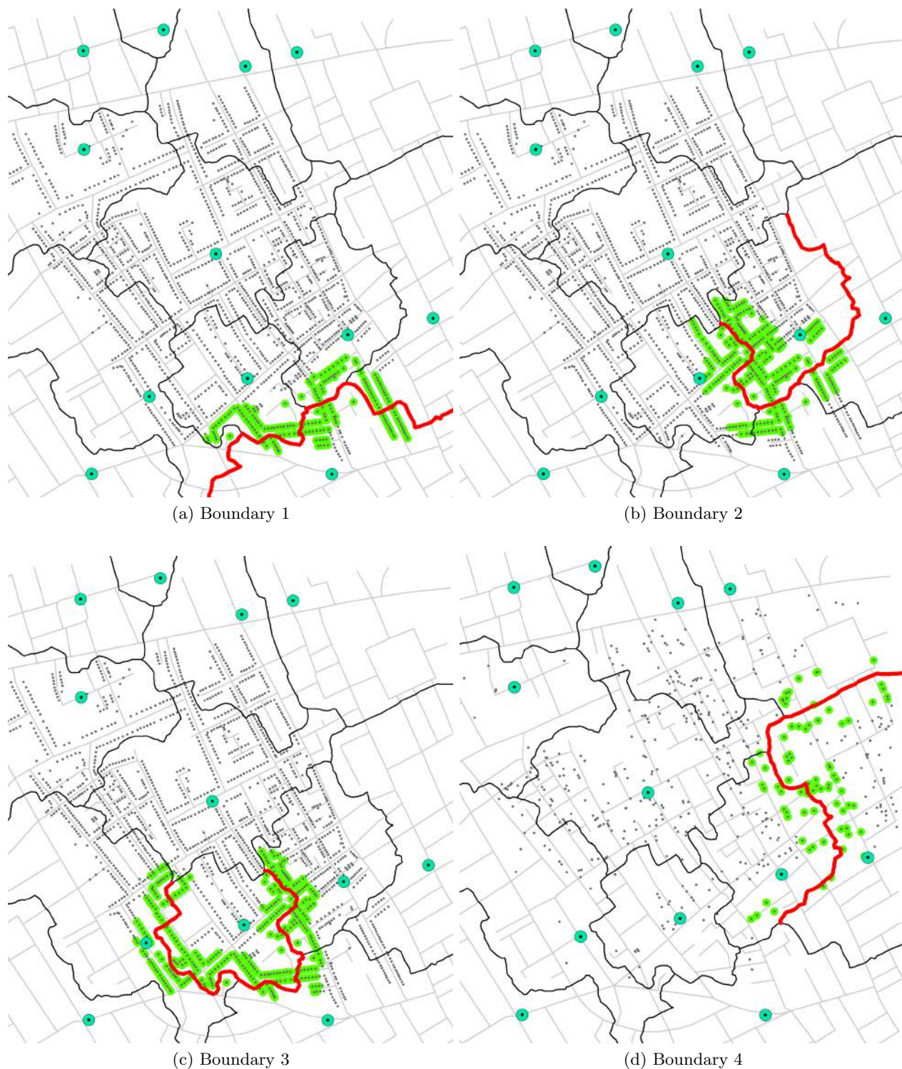
Figure 10: False Treatment Boundaries and Estimation Samples
