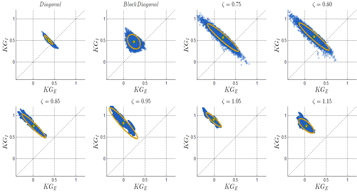
Figure 6: (KG_E, KG_I) Pairs Across MCMC Draws
